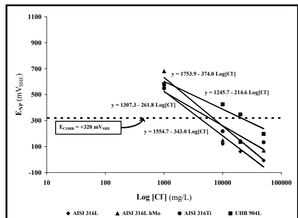
Fig.27: Linear fitting of (E_{\text{NP}}, \log[\text{Cl}^-]) plots of 316L, 316L hMo, 316Ti, and UHB 904L stainless steels in SOCW containing 5,400 mg/L \text{SO}_4^{2-} ( 140^\circ\text{C} ).
