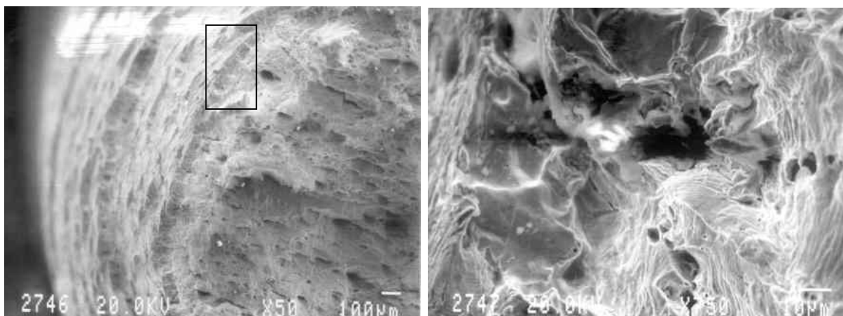
Figure 14: SEM micrographs of the fracture surface of a Cu30Ni alloy specimen tested at a strain rate of 2 \times 10^{-7} \text{s}^{-1} in granitic water with a chloride content of 50000 ppm a) x50, b) x750.
