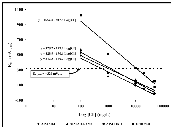
Fig.26: Linear fitting of (E_{\text{NP}}, \log[\text{Cl}^-]) plots of 316L, 316L hMo, 316Ti, and UHB 904L stainless steels in SOCW containing 216 mg/L \text{SO}_4^{2-} ( 140^\circ\text{C} ).
