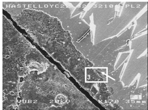
Fig.23: SEM-micrograph of an uncleaned HASTELLOY C-22 sample after CPP-testing in SOCW containing 216 mg/L \text{SO}_4^{2-} and 50,000 mg/L \text{Cl}^- .
