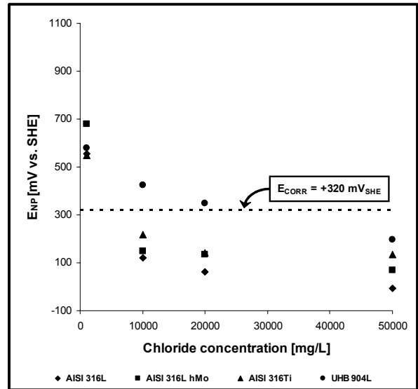
Fig.25: Influence of \text{Cl}^- on E_{\text{NP}} of 316L, 316L hMo, 316Ti, and UHB 904L stainless steels in SOCW containing 5,400 mg/L \text{SO}_4^{2-} .
