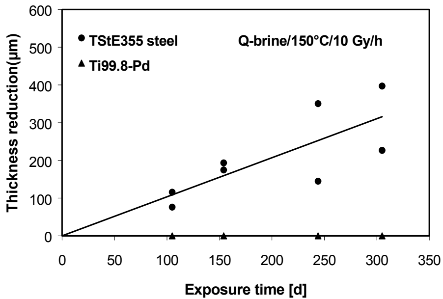
Figure 2: Time-dependence of the thickness reduction of coupled Ti99.8-Pd and TStE355 steel in Q-brine at 150°C and 10Gy/h
