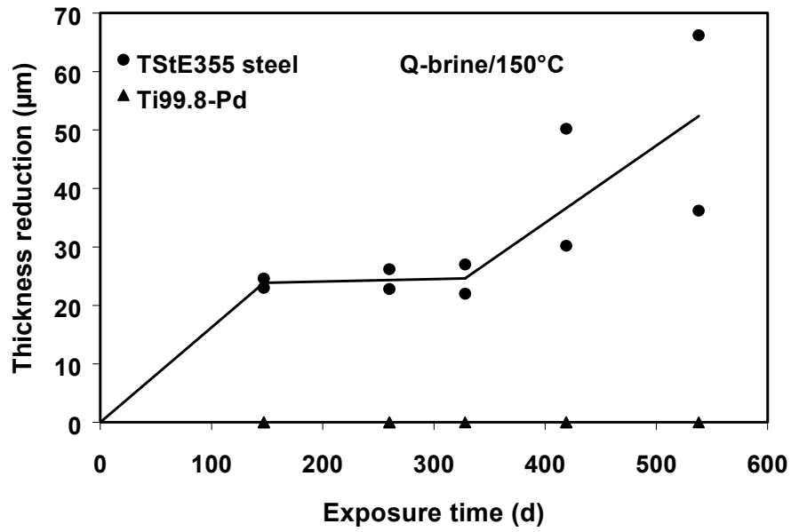
Figure 1: Time-dependence of the thickness reduction of coupled Ti99.8-Pd and TStE355 steel in Q-brine at 150°C
