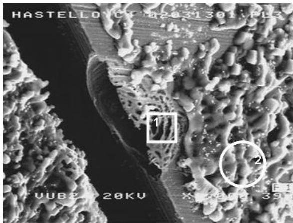
Fig.22: SEM-micrograph of an uncleaned HASTELLOY C-4 sample after CPP-testing in SOCW containing 216 mg/L \text{SO}_4^{2-} and 50,000 mg/L \text{Cl}^- .
