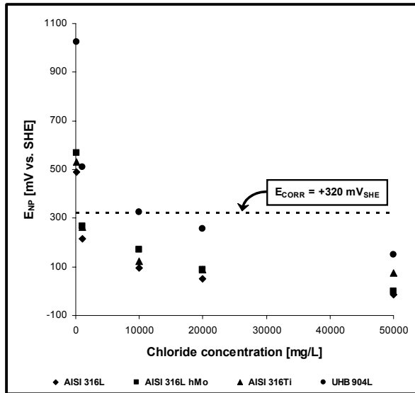
Fig.24: Influence of \text{Cl}^- on E_{\text{NP}} of 316L, 316L hMo, 316Ti, and UHB 904L stainless steel in SOCW containing 216 mg/L \text{SO}_4^{2-} .
